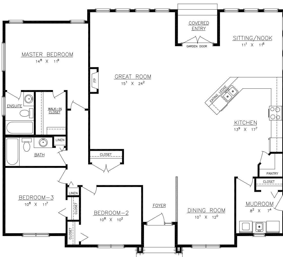
FLOOR PLAN
